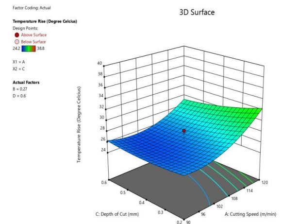
Fig. 3. Interaction effect of cutting speed and depth of cut over temperature rise
